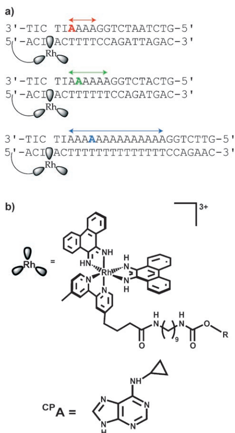
Scheme 1. a) Examples of duplexes used in this study for the \text{CP A} -4, -6, and -14 base-pair series. One position of \text{CP A} is indicated in color and an arrow spans the A tract indicating all employed positions of substitution. b) Structures of the rhodium photooxidant [\text{Rh}(\text{phi})_2(\text{bpy}')_2]^{3+} and the \text{CP A} nucleoside.
