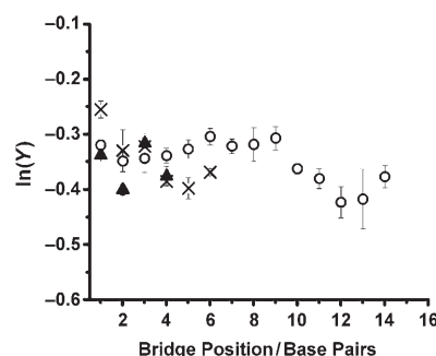
Figure 2. Decomposition ( Y ) as a function of bridge position for \text{CP A} -4 ( \blacktriangle ), -6 ( \times ), and -14 ( \circ ) after irradiation for 30 s at 365 nm. Decomposition was determined by integrating the \text{CP A} peak in the HPLC trace of an irradiated sample relative to that of a nonirradiated sample. Each HPLC trace was normalized to an internal inosine standard. The bars correspond to 2 standard errors for a 95% confidence level (see the Experimental Section).
