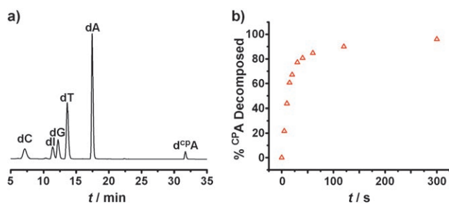
Figure 1. a) Representative HPLC trace monitoring at 260 nm showing the relative retention times of the various deoxynucleosides. b) Plot of \text{CP A} decomposition as a function of irradiation time as determined by HPLC for the 14-base-pair adenine tract in which \text{CP A} is substituted at the first position.
